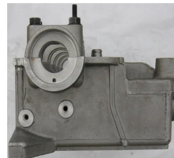
Injectors \varnothing 20mm, Inlet valve \varnothing 40mm, Exhaust valve \varnothing 34mm Valve below the main surface, Inlet & Exhaust valve head recess 1.0 - 1.4mm, square P.C.
