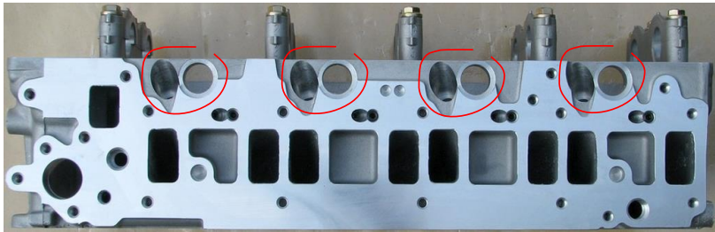
Inlet valve \varnothing 30mm , Exhaust valve \varnothing 28mm
