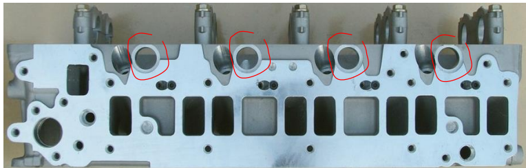
Inlet valve \varnothing 33mm Exhaust valve \varnothing 31mm
